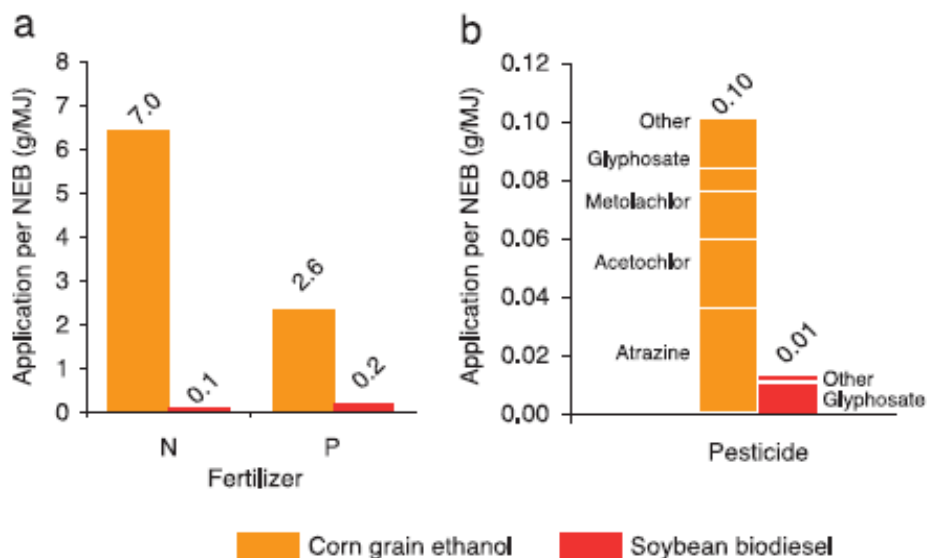
FIGURE 3-5 Environmental effects from the complete production and combustion lifecycles of corn grain ethanol and soybean biodiesel. The figure shows the application of both (a) fertilizers and (b) pesticides, per unit of net energy gained from biofuel production. SOURCE: Hill et al., 2006.
