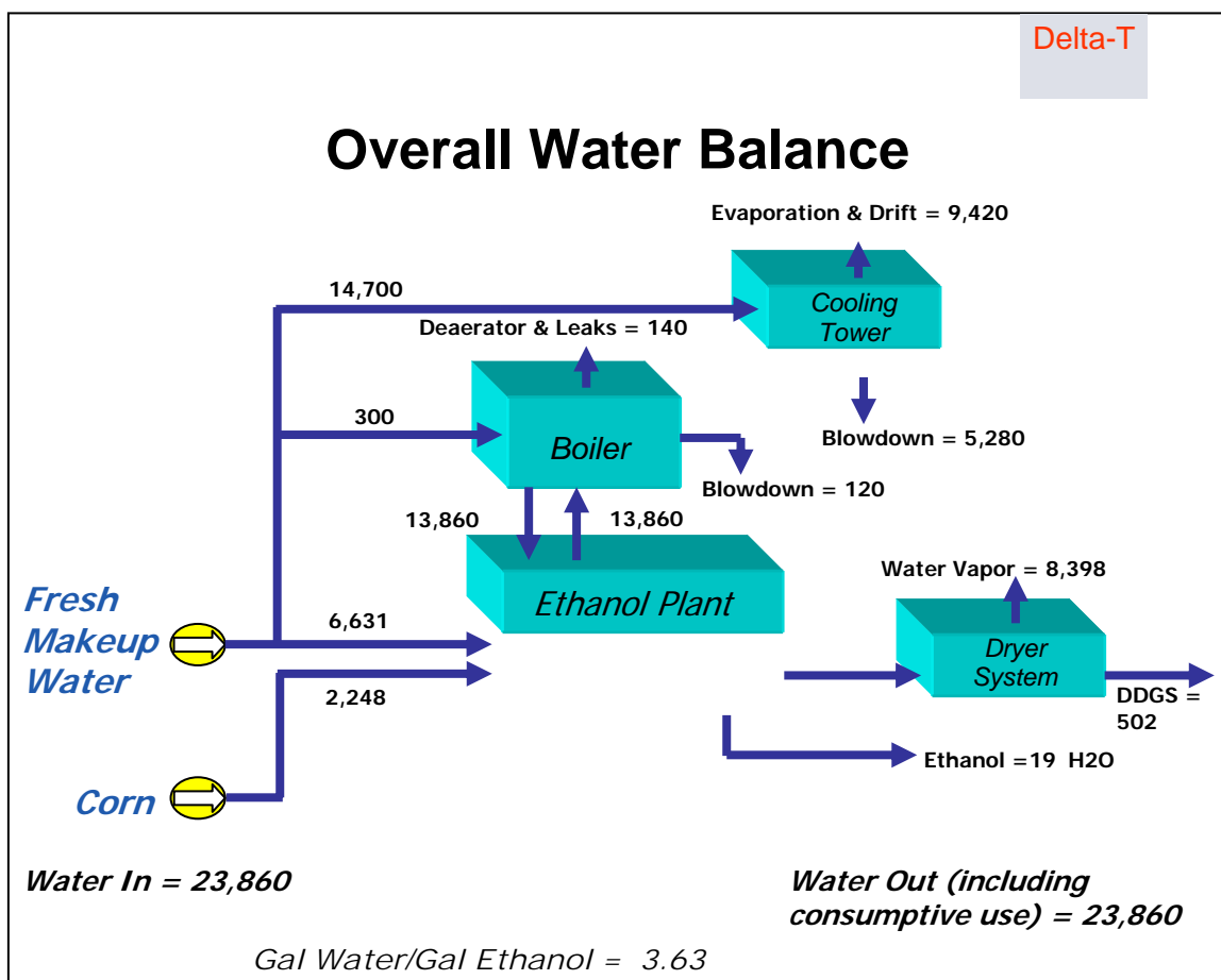
FIGURE 5-2 The overall water balance of a typical 50 million gallon per year corn-based Dry Mill ethanol production facility. All figures are in gallons per hour. SOURCE: Reprinted, with permission, from Courtesy of Delta-T Corp.
